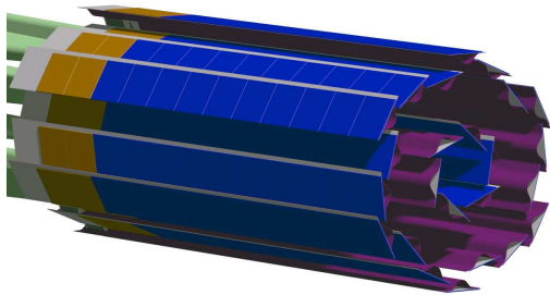
Figure 2. Perspective view of the STAR Heavy Flavor Tracker. The length of the ladders is 20 cm in beam-direction, the two layer radii are 1.5 cm and 5.0 cm, covering full azimuth. The pixel granularity is 100\text{k}/\text{cm}^2 or 100M pixels in total. On the left, the single-sided finger-like support structure is partially visible.
