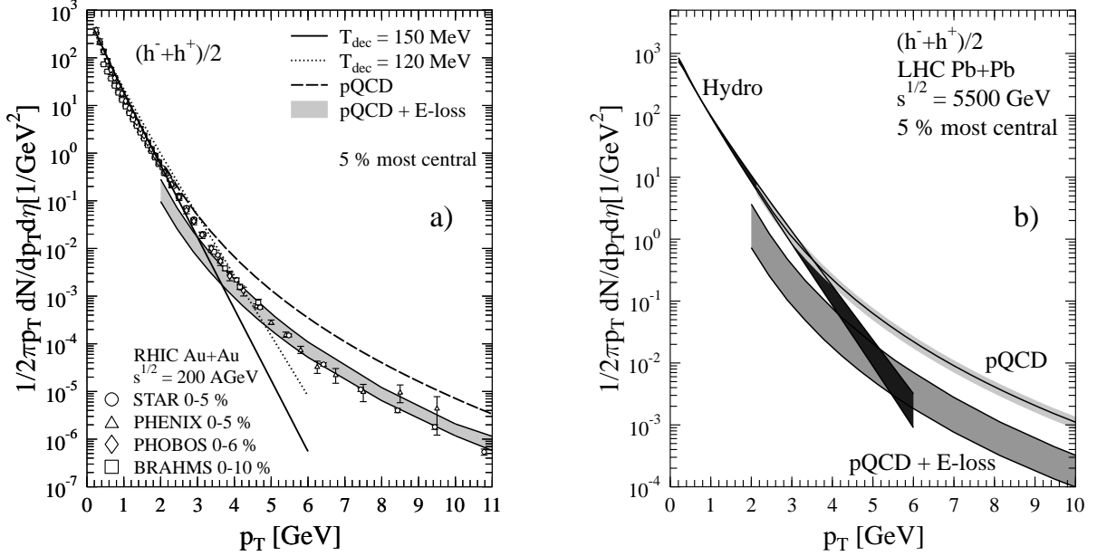
Figure 1. a) Transverse momentum spectra of charged hadrons at y = 0 in 5 % most central Au+Au collisions at \sqrt{s_{NN}} = 200 \text{ GeV} . The solid and dotted lines shows our hydrodynamic results with T_{dec} = 150 \text{ MeV} and T_{dec} = 120 \text{ MeV} respectively. The shaded band shows the pQCD fragmentation+energy loss spectrum and dashed line pQCD fragmentation without energy loss. The data is from Refs. [7–10]. b) As Fig. 1a but for the 5 % most central Pb+Pb collision at \sqrt{s_{NN}} = 5500 \text{ GeV} .
