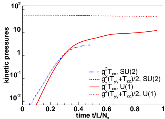
Figure 11. Temporal evolution of the energy-momentum tensor components T^{xx} and (T^{yy} + T^{zz})/2 . The Abelian and non-Abelian results are shown. The figure is taken from [12].
