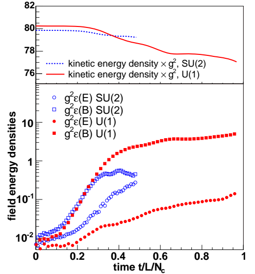
Figure 5. Time evolution of the kinetic energy of particles (upper panel) and of the energy of electric and magnetic fields (lower panel) in GeV/fm 3 for the U(1) and SU(2) gauge groups. The figure is taken from [12].
