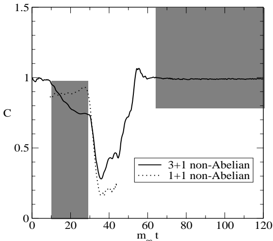
Figure 10. Temporal evolution of the field commutator quantified by C . The figure is taken from [18].
