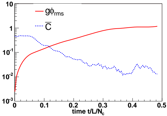
Figure 6. Temporal evolution of the functionals \bar{C} and \phi_{\text{rms}} measured in GeV. The figure is taken from [12].
