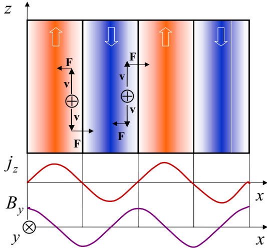
Figure 1. The mechanism of filamentation instability, see text for the description.
