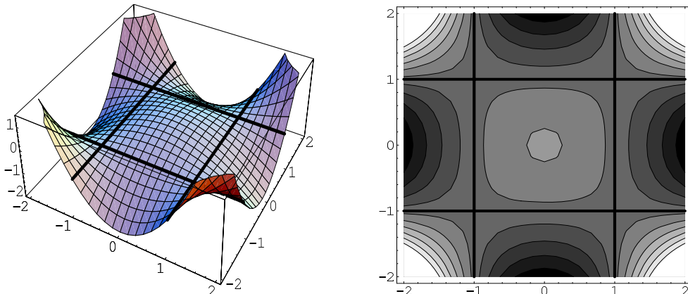
Figure 3. The effective potential of the unstable magnetic mode as a function of magnitude of two colour components of \mathbf{A}^a belonging to the SU(2) gauge group. The figure is taken from [17].
