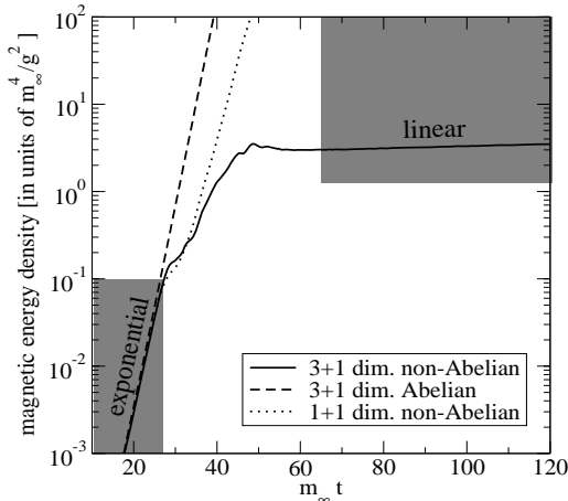
Figure 8. Time evolution of the (scaled) chromomagnetic energy density in the 1+3 dimensional simulation. The Abelian result and that of 1+1 dimensions are also shown. The figure is taken from [18].
