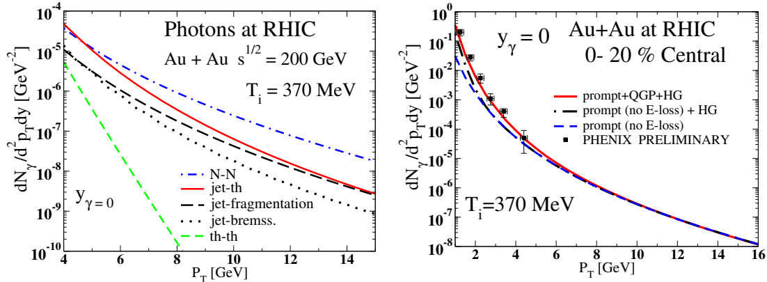
Figure 4. Left Panel: Contributing sources of high- p_T photons at mid-rapidity in central nuclear collisions at RHIC. Solid line: jet-photon conversion in the plasma; dotted line: bremsstrahlung from jets in the plasma; short dashed line: thermal photons [31]; long dashed line: photons from fragmenting jets; dot-dashed line: contribution from the primordial hard scattering. Right panel: Total production of photons at RHIC, compared with new PHENIX data [35]. The solid line represents all processes from the left panel together with photons from the hadronic gas (HG) [31]; the dot-dashed line do not include any plasma-related contributions but has those from the HG. Photons from pp collisions scaled to AA are shown by the dashed lines.
