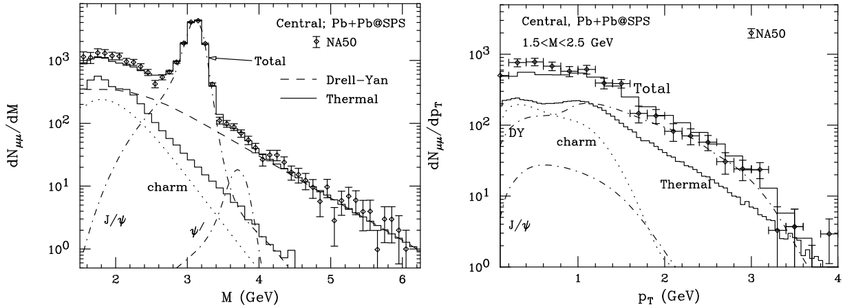
Figure 1. The invariant mass and momentum spectra, calculated for dimuon pairs. The sources are Drell-Yan, correlated charm decay, and thermal (quark-gluon plasma and hadron gas). The full curve histogram is the sum of all of those different contributions, after correcting for detector acceptance, resolution, and efficiency.
