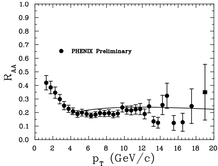
Figure 3. The ratio R_{AA} for \pi^0 , as a function of transverse momentum. The full line is the calculation described in this text, and in [29], with \alpha_s = 0.34 . The initial temperature is 370 MeV, and is consistent with the study in [31]. Data are from [32].
