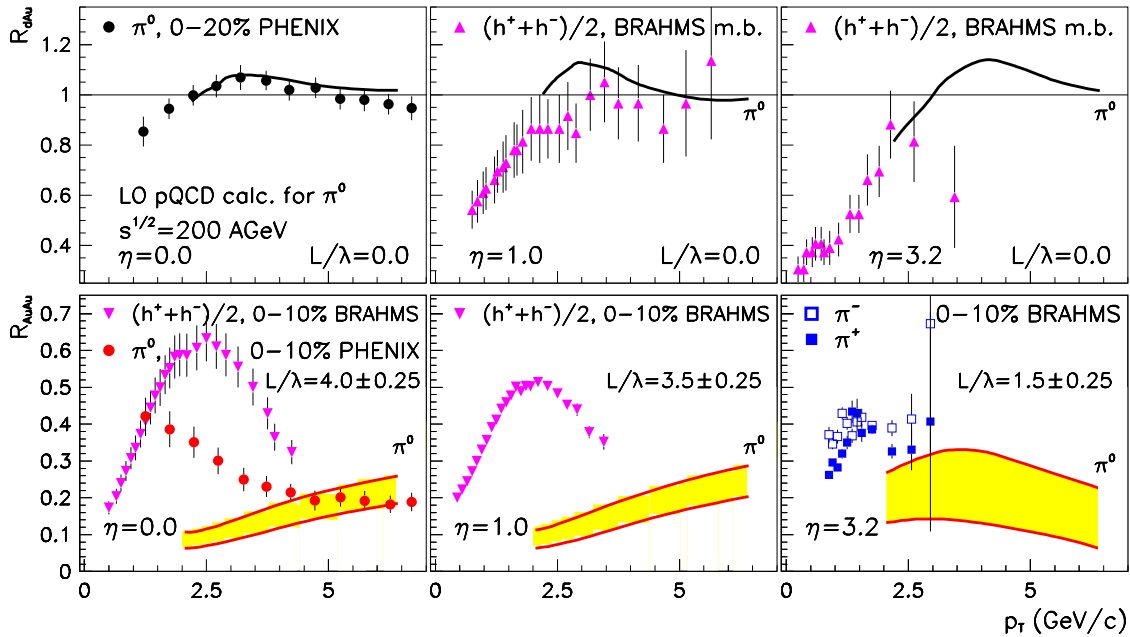
Figure 1. Nuclear modification factors at different rapidities: R_{dAu}^\pi in dAu collisions (upper row), R_{AuAu}^\pi in 0 – 10% central AuAu collisions (lower row). Data are from PHENIX [1,12] and BRAHMS [3,13] at \sqrt{s} = 200 AGeV. Full lines display our pQCD results, the bands indicate the theoretical uncertainties on the value of the opacity.
