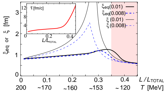
Figure 3: Equilibrium correlation length \xi_{\text{eq}} and non-equilibrium correlation length \xi on the isentropic trajectories with n_B/s = 0.008 and 0.01 , together with \tau as functions of L/L_{\text{total}} (inlet).
