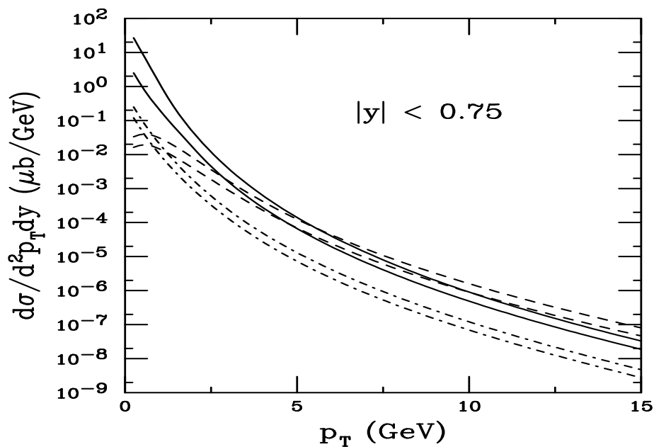
Figure 11: The theoretical FONLL bands for D \rightarrow eX (solid), B \rightarrow eX (dashed) and B \rightarrow DX \rightarrow eX' (dot-dashed) as a function of p_T in \sqrt{S} = 500 GeV pp collisions for |y| < 0.75 .
